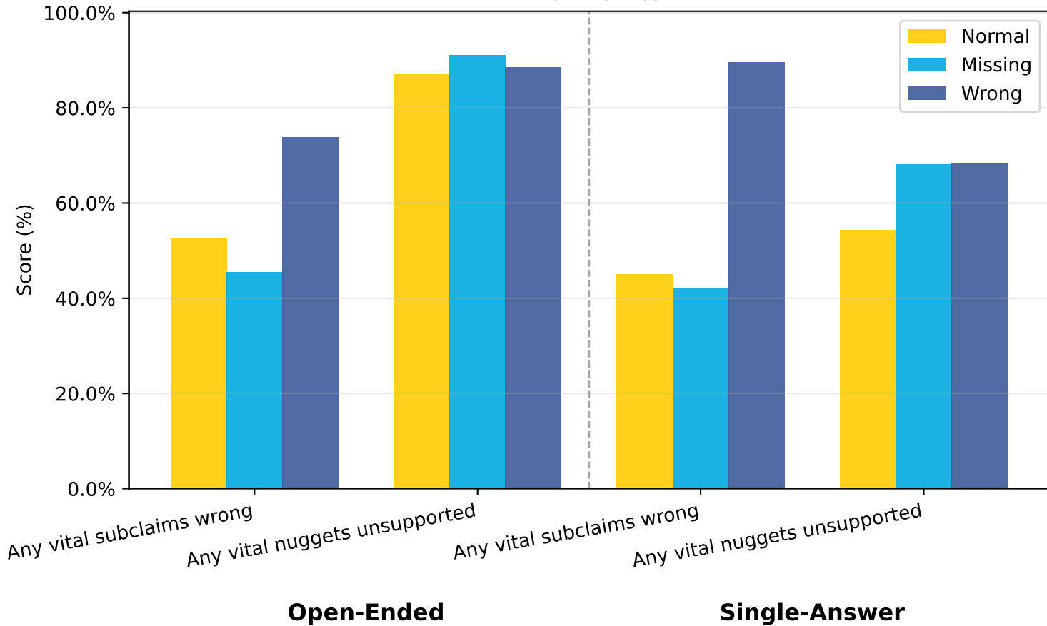
Error Metrics
